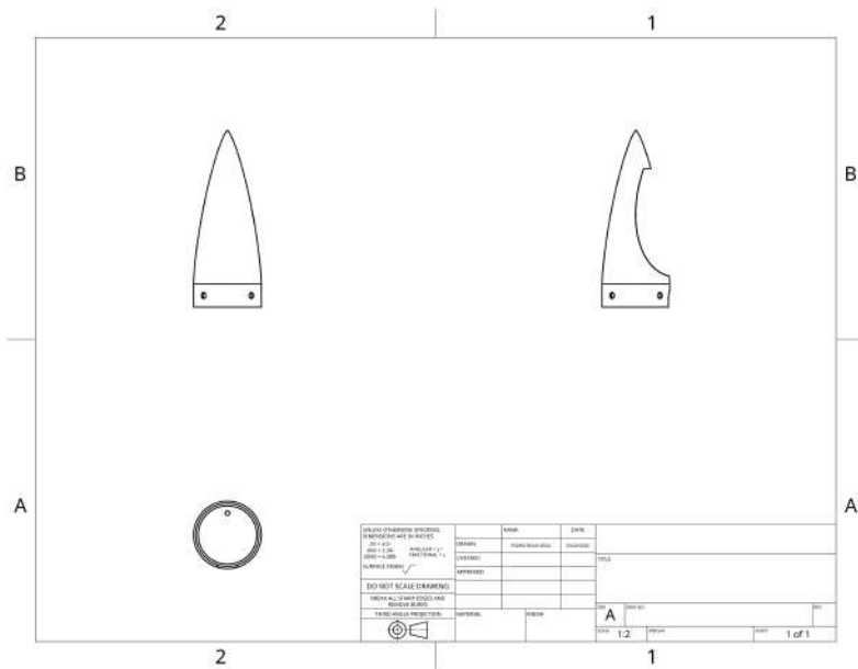
Figure 5: Nose Cone and Parachute Bay Assembly
