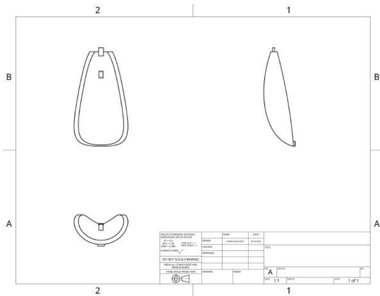
Figure 6: Parachute Bay Cover
