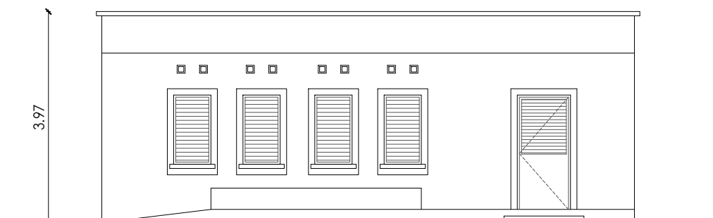
FAÇADE PRINCIPALE
