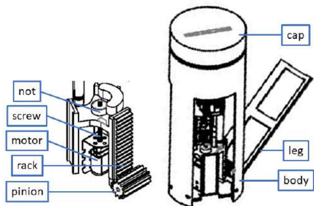
Figure 5 : main mechanical pieces of the CanSat
